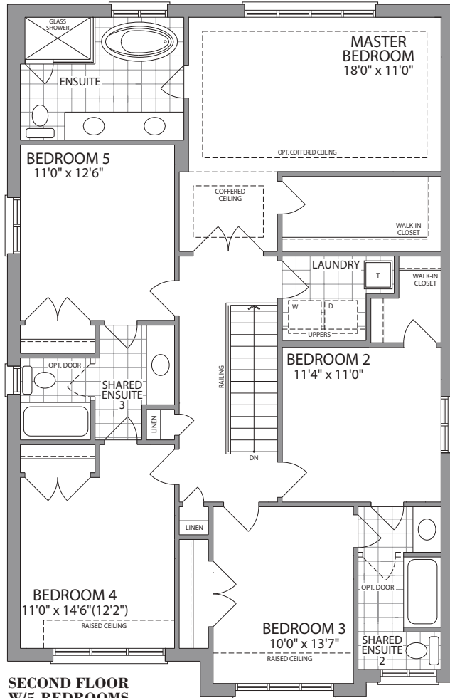
ELEVATION A ~ 2814 SQ. FT.
