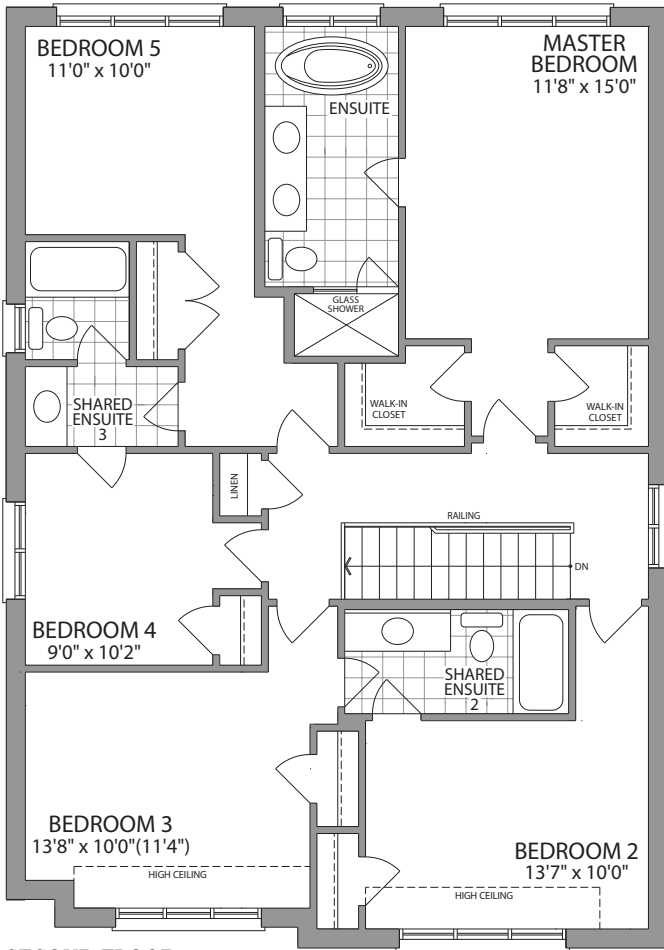
SECOND FLOOR W/5 BEDROOMS ELEVATION A
