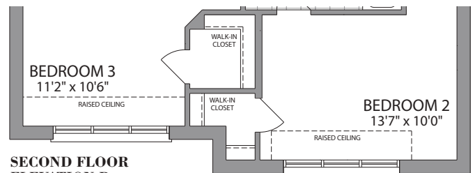
SECOND FLOOR ELEVATION A
